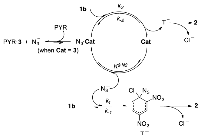
Scheme 2. Mechanistic Proposal for the Catalyzed S_NAr Reaction between 1b and NaN_3 ; The Inhibitory Effect Observed upon Addition of Pyrene (PYR) for Cat = 3·6NO 3 Is Also Represented
