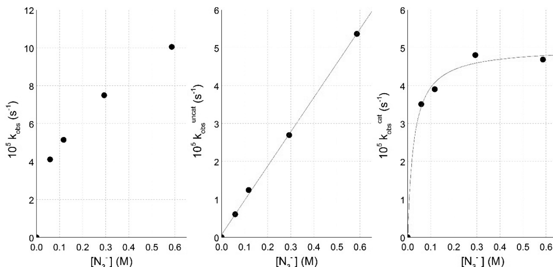
Figure 2. Influence of azide ion concentration on the overall (left), uncatalyzed (middle), and catalyzed (right) observed rate constants for the S_NAr reaction between 1b and NaN_3 in D_2O/CD_3CN (4:1), where k_{obs} = k_{obs}^{uncat} + k_{obs}^{cat} , [1b] = 6 \text{ mM} ; [3\cdot 6NO_3] = 0.6 \text{ mM} (10 mol %); T = 25^\circ \text{C} .
