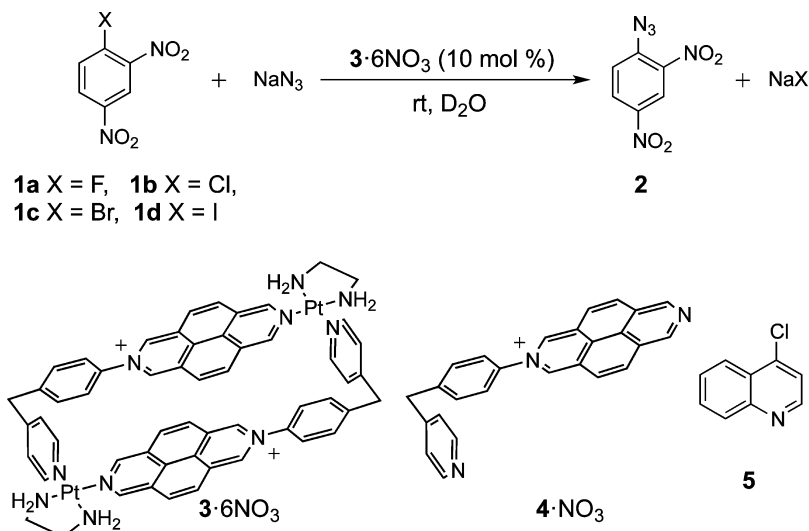
Scheme 1. Model S_NAr Reaction and Species Discussed in This Work
