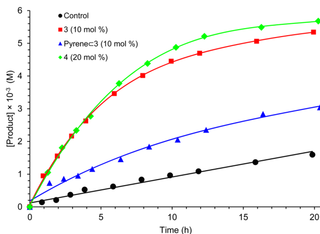
Figure 1. Kinetic data for the S_NAr reaction between 1b (6 mM) and NaN_3 (60 mM) in D_2O/CD_3CN (4:1) at rt in the presence of 3·6NO 3 (0.6 mM, 10 mol %) (red ■), 4·NO 3 (1.2 mM, 20 mol %) (green ◆), or metallacycle 3·6NO 3 (0.6 mM, 10 mol %) + pyrene (blue ▲) or in the absence of catalyst (black ●) as a control.
