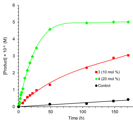
Figure 3. Kinetic data for the \text{S}_{\text{N}}\text{Ar} reaction between 5 (6 mM) and \text{NaN}_3 (60 mM) in \text{D}_2\text{O}/\text{CD}_3\text{CN} (4:1) at rt in the presence of 3·6NO 3 (0.6 mM, 10 mol %) (red ■) or 4·NO 3 (1.2 mM, 20 mol %) (green ◆) or in the absence of catalyst (black ●) as a control.
